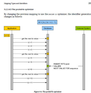
Figure 9.4 The pooled-to optimizer If increment size (n) is the number of identifiers within a range, the pooled-to optimizer will generate identifiers with the following formula: id = (id - n) + (n * i) . • The first sequence call generates the hi value, so the first range of identifiers is (1, 2, 3). • When adding the 3th entry, the pooled-to optimizer calls the sequence and obtains the next hi value, the next identifier range being (4, 5, 6). • After inserting the 3th entry, an external system adds a post row and assigns the primary key with the value returned by the sequence call. • The Hibernate application the read resumes and inserts the identifier 6. • The 7th entry requires a new sequence call, and so a new range is allocated (10, 11, 12).
